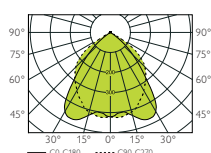
BASIC II 2x1L RT600 T5 2x28W PSL MIRO4
