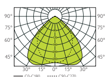
BASIC II 2x1L RT600 T5 2x28W PML
