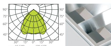
BASIC II 2x1L RT600 T5 2x28W PML MIRO5
