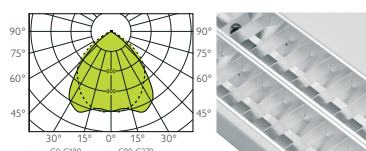
BASIC II 2x2L RT600 T5 4x14W PML MIRO5
