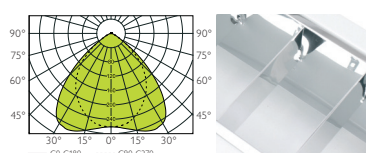
BASIC II 1x1L RT600 T5 1x28W PML
