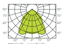
BASIC II 1x4L RT600 T5 4x14W PSL MIRO4
