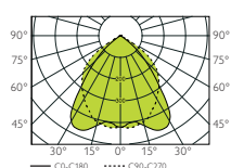
BASIC II 1x1L RT600 T5 1x28W PSL MIRO4
