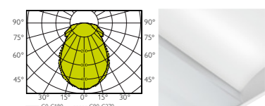
JAZZ RT600 LED 3260lm
